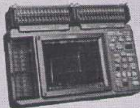
MEMORY HILOGGER LR8401-20 30 isolated analog input channels With built-in UNIVERSAL UNIT × 2 modules
