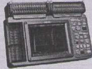
MEMORY HILOGGER LR8402-20 30 isolated analog input channels With built-in UNIVERSAL UNIT × 1, VOLTAGE TEMP UNIT × 1 modules
