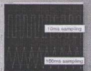
Measurement comparison of 5kHz square pulse waveform with 10 ms (upper trace) and 100 ms sampling
