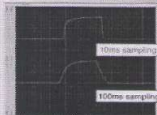
Measurement comparison of abrupt load change in waveform with 10 ms (upper trace) and 100 ms sampling
